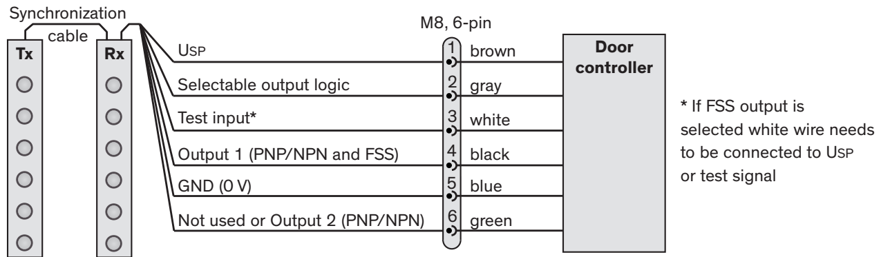
Figure 11: Connection diagram
