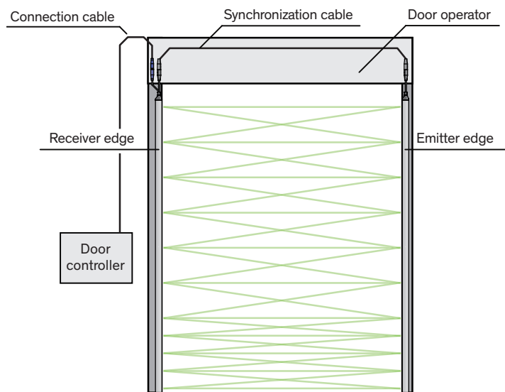
Figure 6: GridScan/Pro application (overview)
