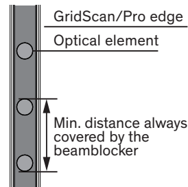
Figure 9.2 Door blanking through beam blocker
