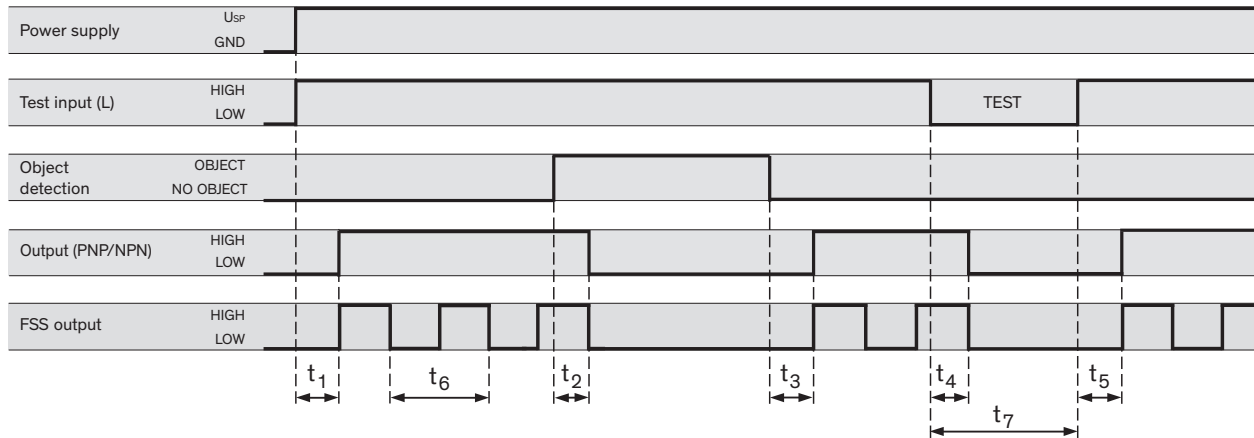
Figure 13: General timing diagram
